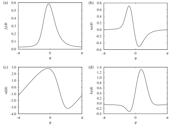
FIG. 3. (a) Distribution function f_0(\phi) . (b) Right zero eigenfunction u_0(\phi) . (c) Left zero eigenfunction u_0^*(\phi) . (d) Kernel function k_0(\phi) . Parameters are D=D_c/2=(\cos \alpha)/4 and \alpha=3\pi/8 , where order parameter amplitude is R=0.653\ 28 . \beta=3\pi/8 gives \rho \cos \delta=-0.322\ 64 , whereas \beta=-5\pi/8 gives \rho \cos \delta=0.322\ 64 .
