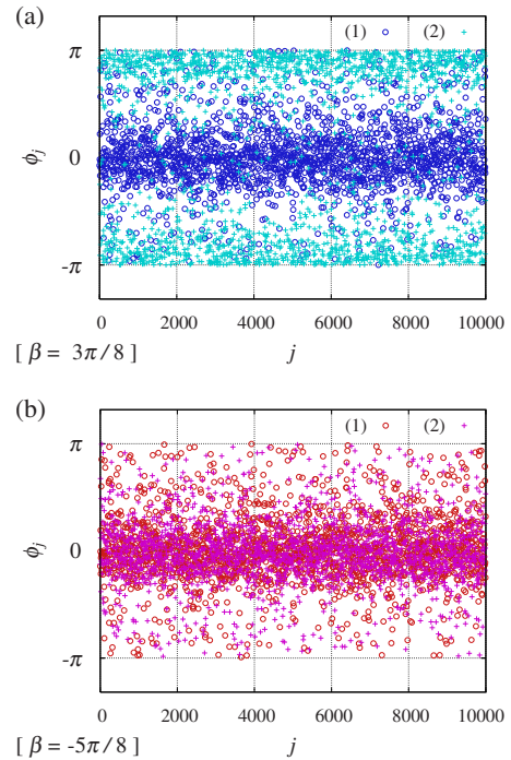
FIG. 2. (Color online) Snapshots of the asymptotic states of the individual oscillators in Fig. 1. Only one in every five oscillators is plotted. Open circle (○) and plus (+) respectively indicate oscillator of group (1) and that of group (2). (a) Effective antiphase coupling with microscopic in-phase coupling, \beta = 3\pi/8 . (b) Effective in-phase coupling with microscopic antiphase coupling, \beta = -5\pi/8 .
