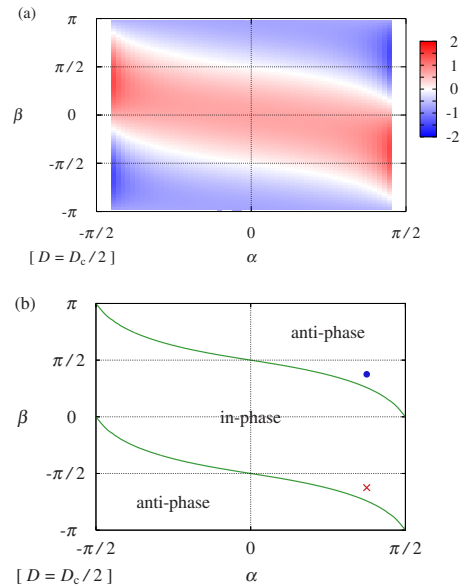
FIG. 4. (Color online) Effective type of phase coupling between collective oscillations with \alpha \in (-\pi/2, \pi/2) , \beta \in [-\pi, \pi] , and D=D_c/2=(\cos \alpha)/4 , which is numerically evaluated by Eq. (24). (a) Dependence of \rho \cos \delta on \alpha and \beta . (b) The solid curves are determined by \rho \cos \delta=0 . The filled circle (●) indicates \alpha=\beta=3\pi/8 corresponding to Figs. 1(a) and 2(a). The cross (×) indicates \alpha=3\pi/8 and \beta=-5\pi/8 corresponding to Figs. 1(b) and 2(b).
